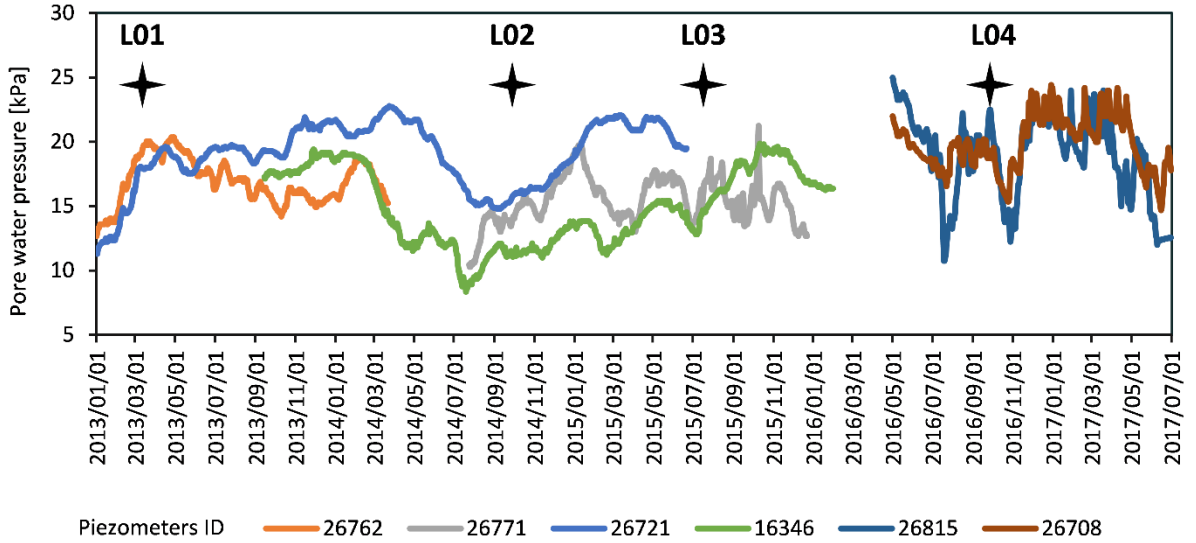
Figure 5. Pore-water pressures recorded in the 6 considered piezometers in the period of analysis (dates with landslides are indicated with cross marks)
