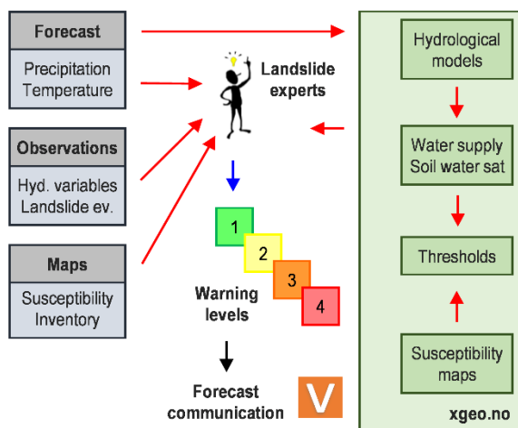
Figure 1. Conceptual framework of the national LEWS (red arrows indicate quantitative processes; blue arrow indicates a qualitative process)
